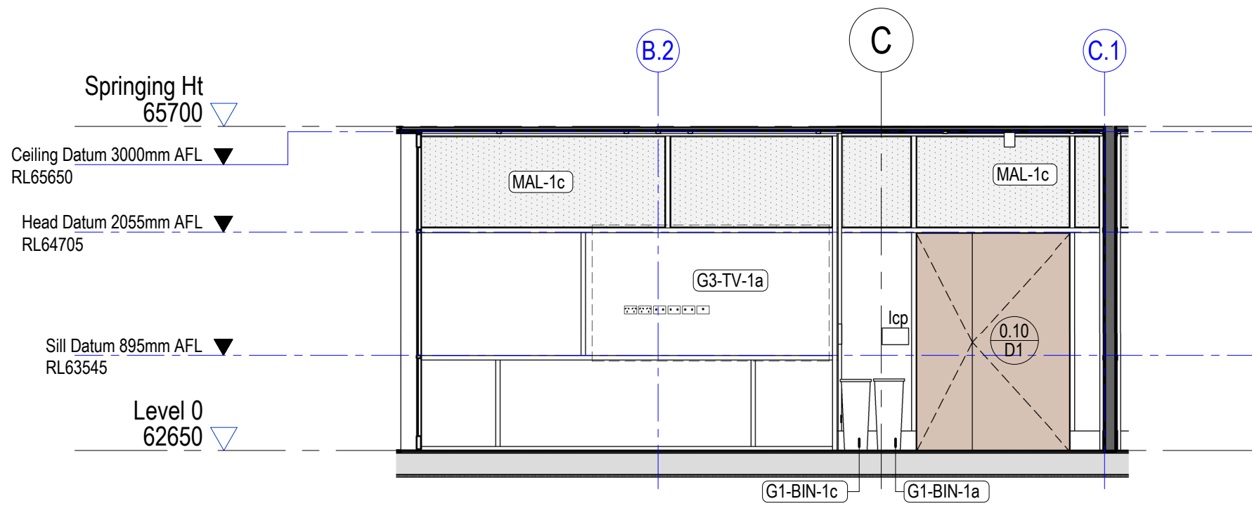
2 0.10 - Training 01 - North Elevation 1 : 50
