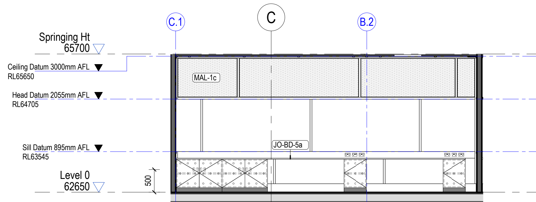
4 0.10 - Training 01 - South Elevation 1 : 50
