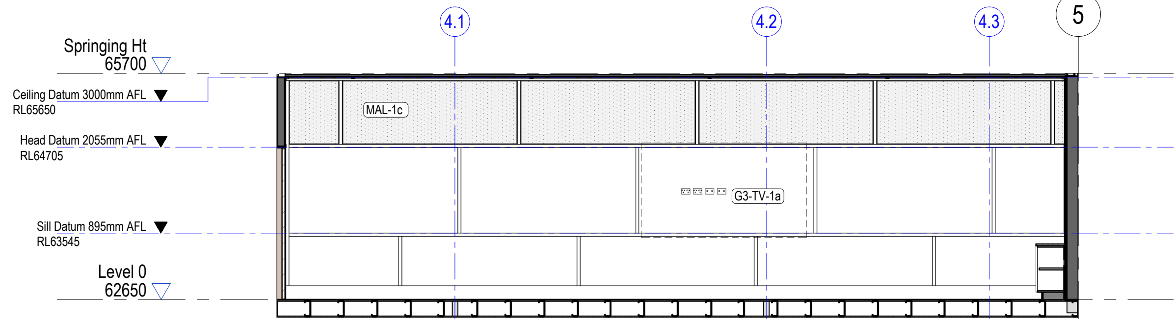
3 0.10 - Training 01 - East Elevation 1 : 50
