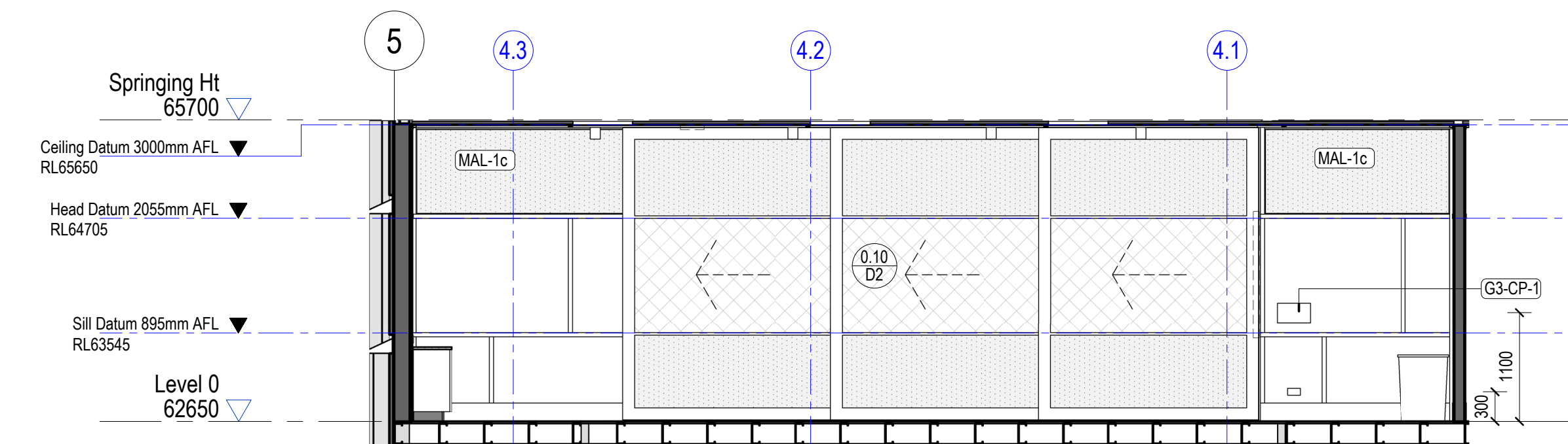
5 0.10 - Training 01 - West Elevation 1 : 50
